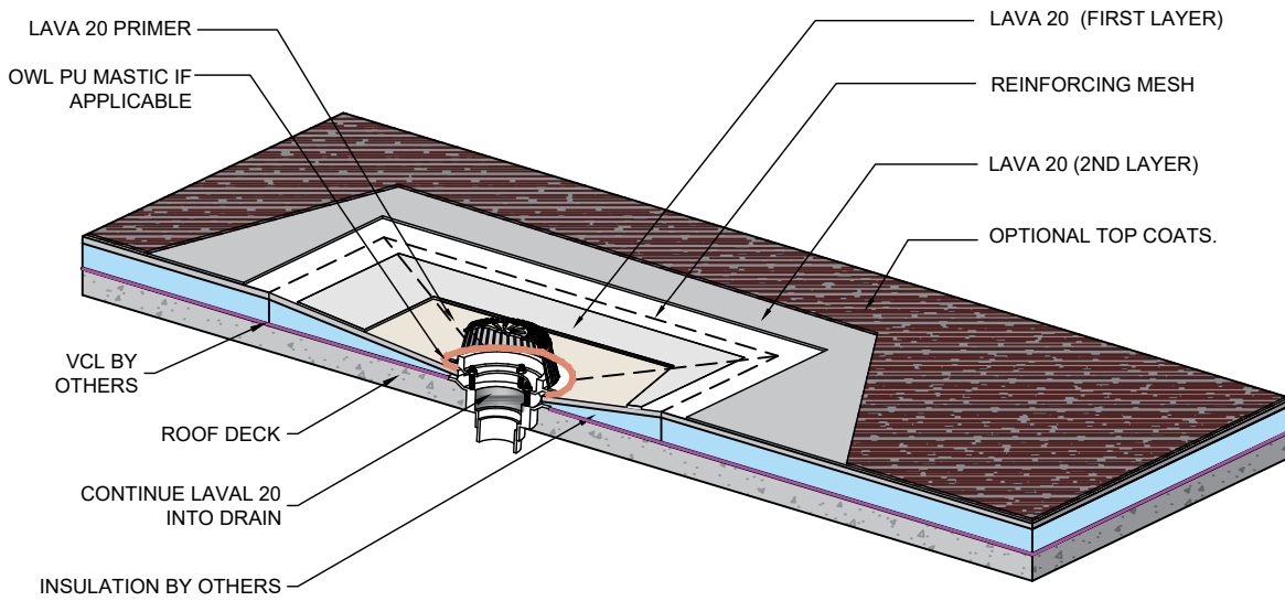
ISOMETRIC SECTION
